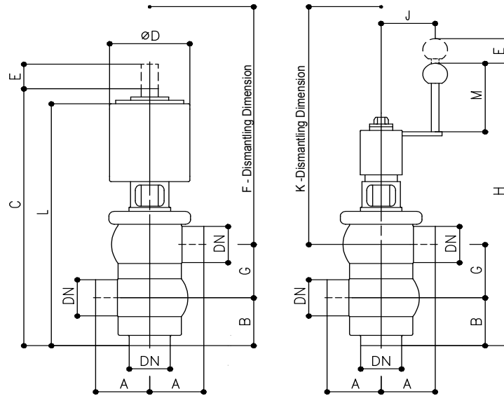
Changeover Valve 3x Welding End
